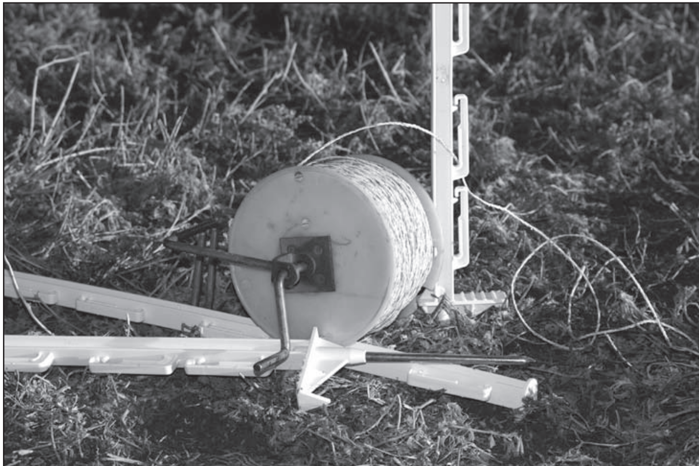
For faster construction, particularly when temporary fences will be moved frequently, producers may want to consider plastic "tread-in" posts. These feature a spike on the bottom and a tread-plate on which the fence-builder places his or her foot to push the post into the ground.
